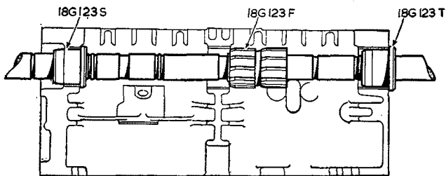
18G123A. Camshaft Liner Reamer (basic tool), Cutters, and Pilots
